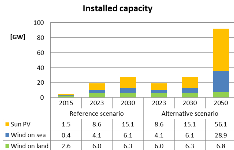
Figure 8: Assumed installed capacity, full load hours and resulting electricity output by VRE power sources in all scenario cases, 2015-2050
