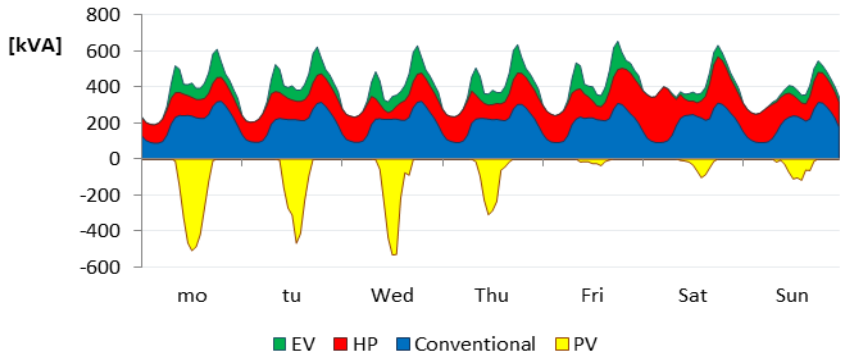
Figure 39: Demand & supply profiles and residual load for a winter and summer week at a MV/LV distribution transformer in the alternative scenario case 2050 (A2050)
