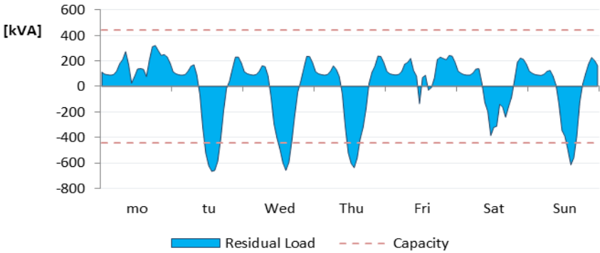
Power load summer (week 30)
