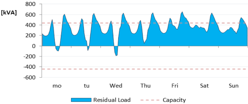
Power load winter (week 6)
