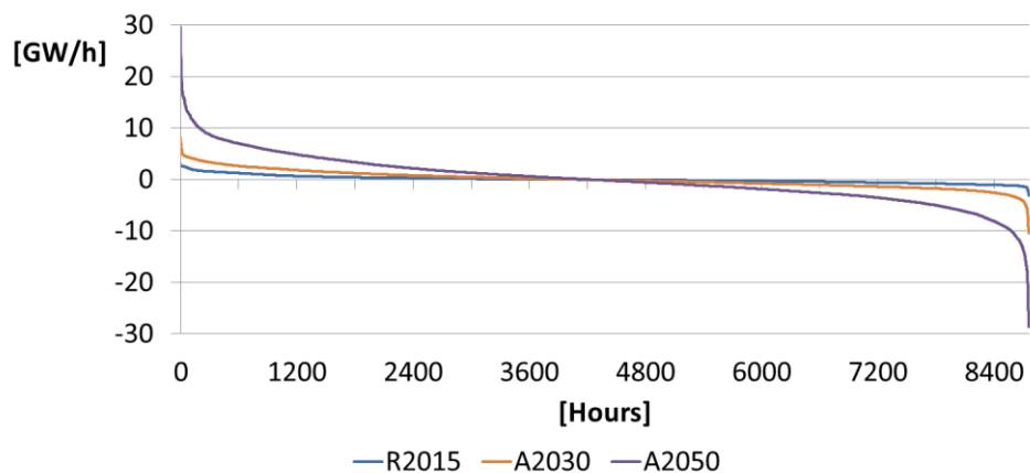
Figure 23: Ramp duration curve of the residual load in three scenario cases, 2015-2050
