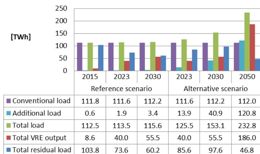
Figure 54: Total annual power load and VRE electricity generation in all scenario cases, 2015-2050
