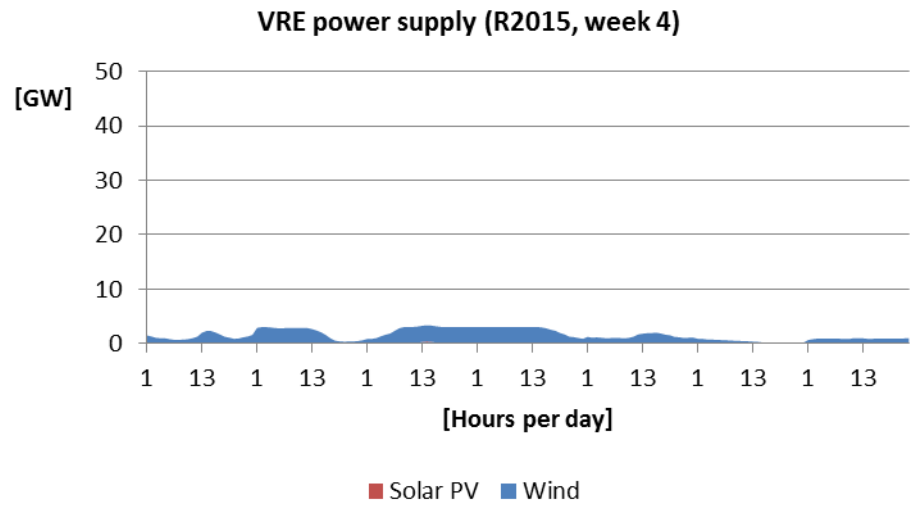
Figure 12: VRE power supply during week 4 in some scenario cases, 2015-2050
