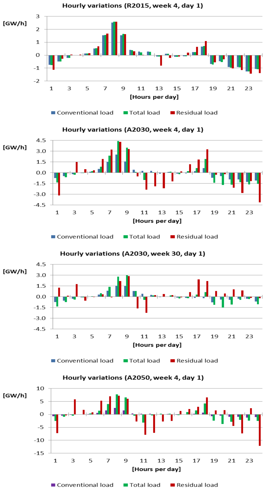
Figure 22: Hourly variations ('ramps') of conventional load, total load and residual load during the first day (Monday) of weeks 4 and 30 in selected scenario cases, 2015-2050
