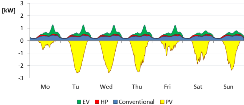
Figure 38: Demand & supply profiles and residual load for a winter and summer week for a single household in the reference scenario case 2015 (R2015)
