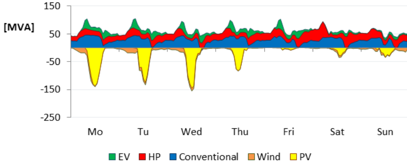
Figure 41: Demand & supply profiles and residual load for a winter and summer week at the Zaltbommel substation in the alternative scenario case 2050 (A2050)
