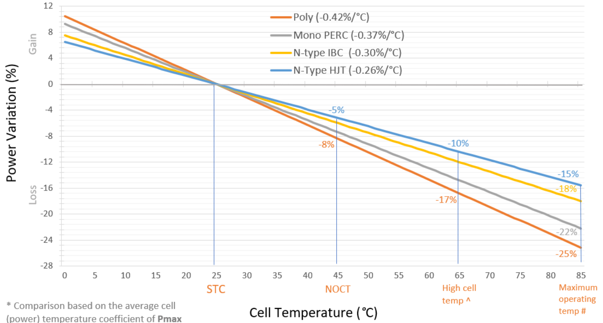
Solar module - Power Vs Temperature *
