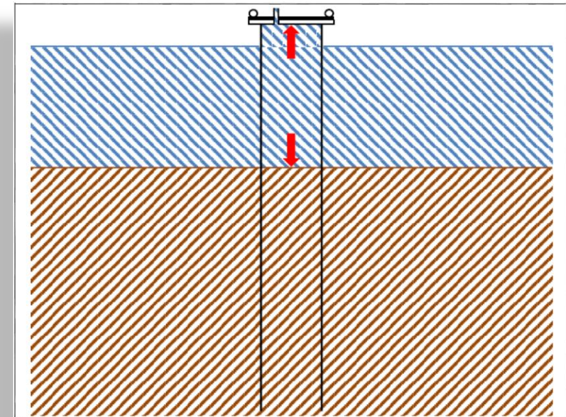
Figure 2. Illustration of hydraulic pile extraction (source: innogy)
